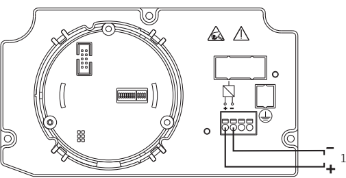
1 FOUNDATION fieldbus™ o PROFIBUS® PA
