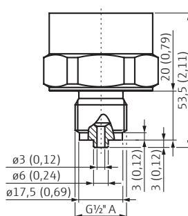
Rosca ISO 228 G \frac{1}{2} "
