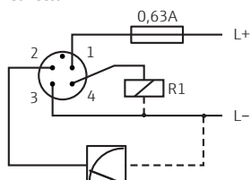
Conector M12
